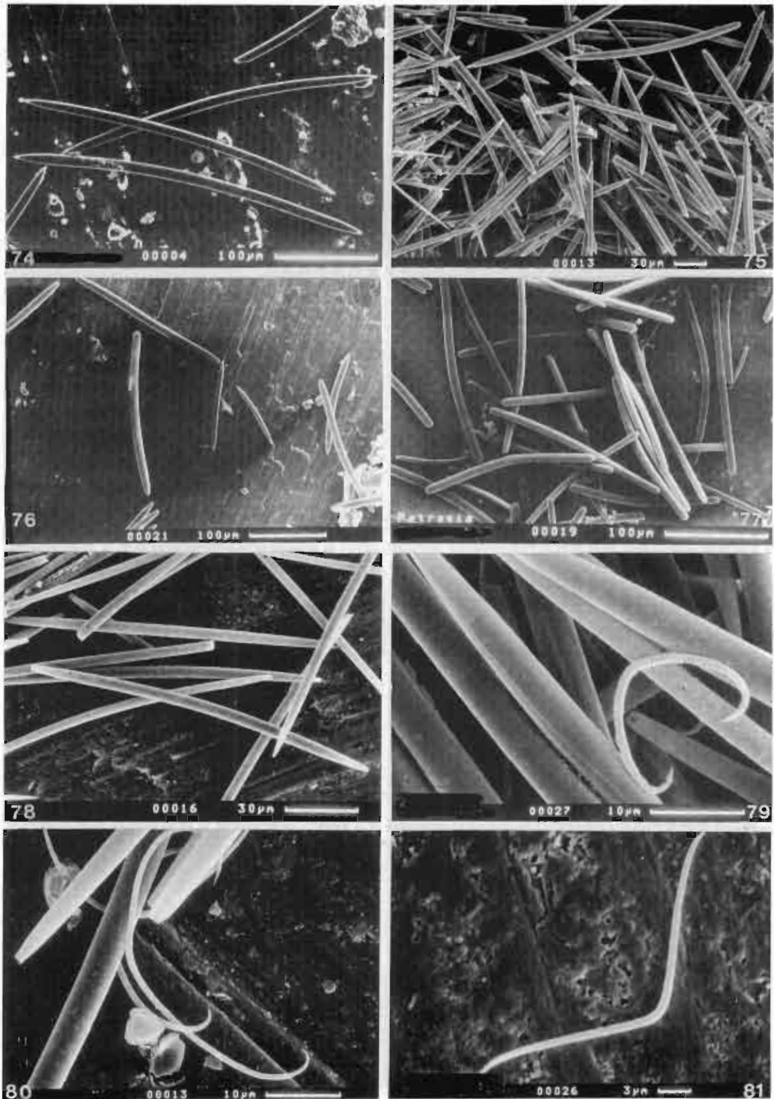
Figure 1. Scanning electron micrographs of the nematode Paratrichia sp. n. (74-81).
