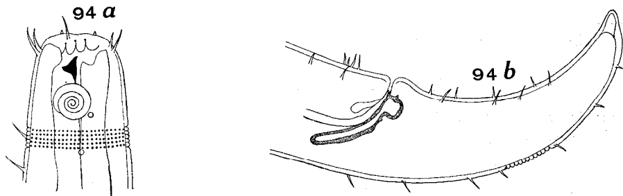
Paracanthonchus kreisi ALLGÉN a. Head, b. Tail and spicules, \times 450
