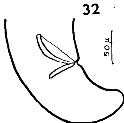
32. Pontonema serratodentatum : tail of male.
