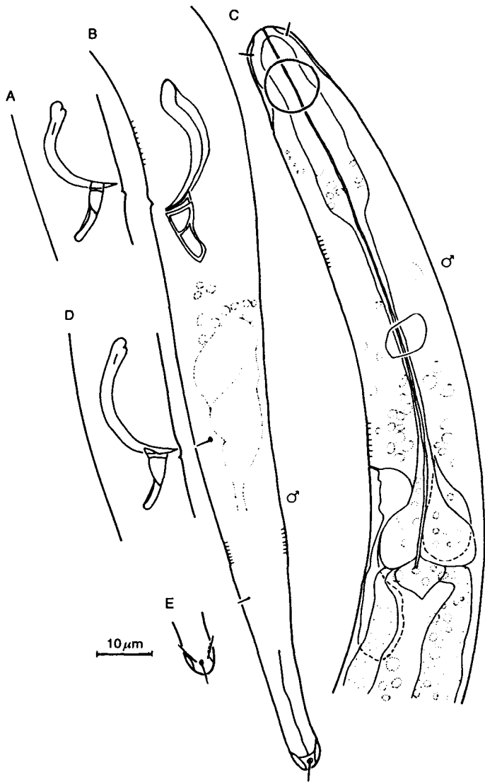
Fig. 215. Cyartonema germanicum . A, Cloacal region; B, Male tail; C, Anterior end of male; D, Cloacal region of another specimen; E, Tail tip. From Juario (1972).
