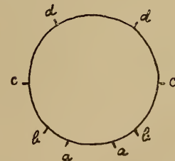
TEXT-FIG. 1.— Comarodrilus gravelyi ; ideal transverse section, to show setal distribution in pre-clitellar region.
