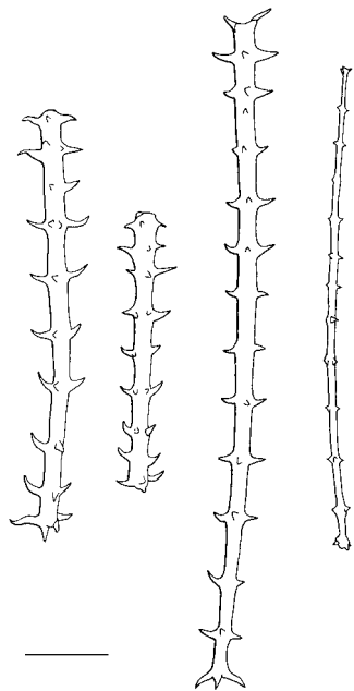
Fig. 3. Goreauiella auriculata Hartman, 1969. Siliceous strongyles (scale 12.3 \mu\text{m} ), from Hartman (1969).
