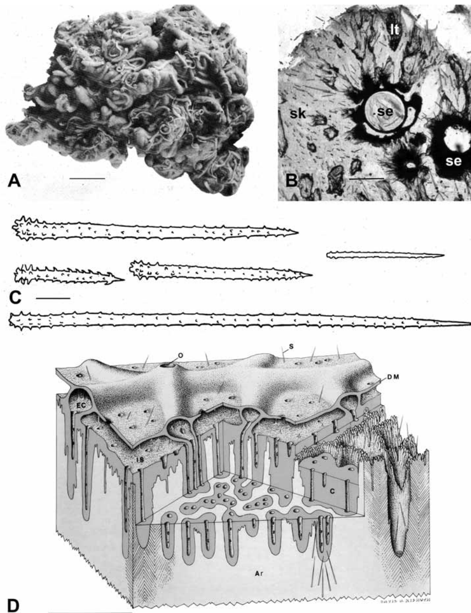
Fig. 5. Stomatosporgia vermicola Hartman, 1969. A, holotype YPM 6376 (scale 16.5 mm), from Hartman (1969). B, polished section through a specimen from Jamaica; lt: living tissue; se: tube of serpulid worms; sk: calcareous skeleton with siliceous verticillately spined styles (scale 312 \mu m). C, acanthostyles (scale 30 \mu m), from Hartman (1969). D, three dimensional schematic representation; Ar: aragonitic skeleton; c: choanosome; DM: dermal membrane; EC: exhalant canal; IS: inhalant space or vestibule; O: osculum; S: spicule (scale 1 mm), from Willenz & Hartman (1989).
