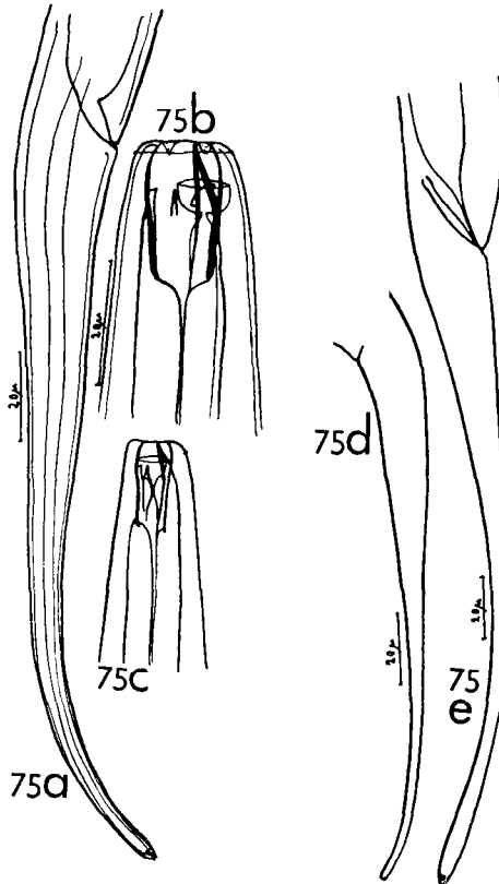
Fig. 75: Viscosia carnleyensis : a — tail of female, b — anterior end of female, c — anterior end of juvenile, d — tail of juvenile, e — tail of male.
